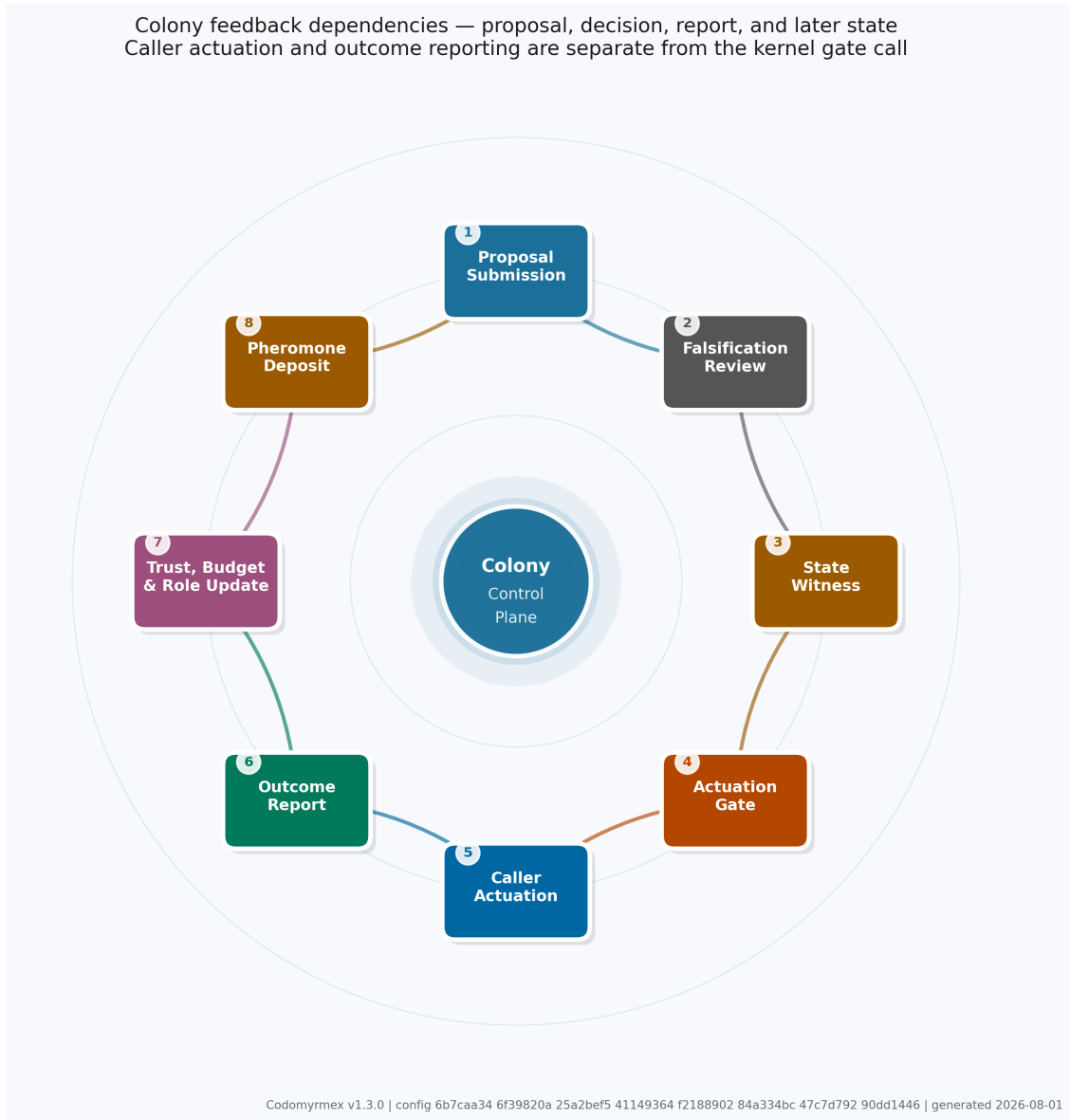
Figure 6: Conceptual Colony Kernel feedback dependencies. Proposal review reads budget, local RISK/FAILURE pressure, role, trust, and completeness; a separate caller may execute an approved action and report its outcome; recording then changes trust, resource usage, and signal traces used on a later proposal. Arrows show feedback dependencies rather than exact runtime call order.
