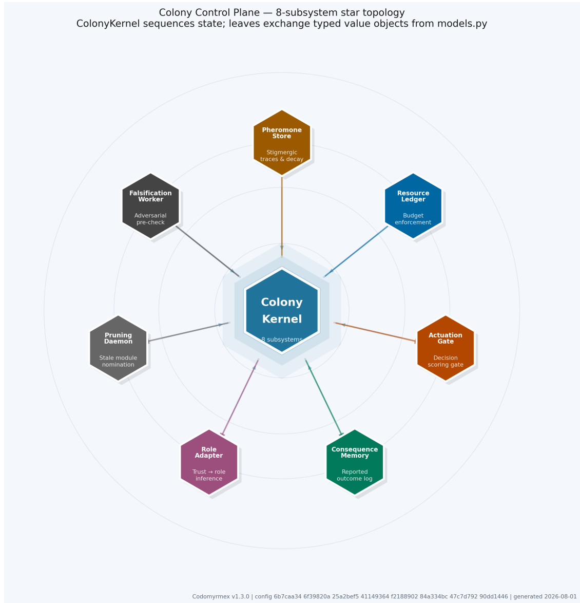
Figure 4: Colony Control Plane topology. ColonyKernel owns subsystem lifecycle and sequencing; the live integration object supplies the operational leaf-node count, and the nodes exchange typed value objects from the shared models.py contract. Node labels, radial position, and arrow direction identify each functional role; colour is a secondary cue. The diagram shows ownership and information flow, not deployment topology or performance.
