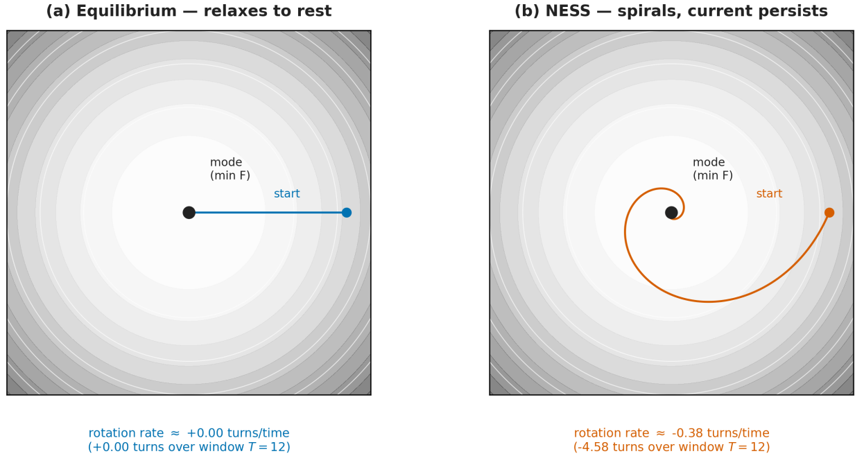
Figure 3: Worked trajectories over one landscape. Both panels integrate the Bayesian-mechanics flow \dot{f} = (Q - \Gamma)\nabla F from the same starting point (coloured dot) over the same Gaussian free-energy bowl (grey contours; black dot marks the mode). (a) Equilibrium ( Q = 0 ): pure descent falls radially to the mode and rests — free energy monotonically decreasing, rotation rate \approx 0 turns/time. (b) NESS ( Q \neq 0 ): the same descent plus a solenoidal term spirals inward at a constant rate \approx -0.38 turns/time ( \approx -4.58 turns over the window T = 12 ) while free energy still decreases monotonically. The nonzero rotation rate witnesses the broken detailed balance in the corresponding stochastic model; sec. 8 computes its stationary probability current. Rendered deterministically by scripts/generate_trajectory_figure.py over the tested cores in src/trajectories.py and src/free_energy_flow.py .
