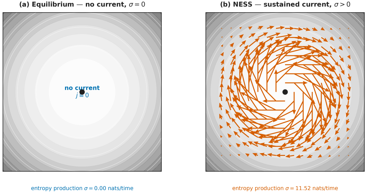
Figure 6: Probability current and entropy production. Both panels place the same stationary Gaussian density (grey contours) under the Bayesian-mechanics diffusion. (a) Equilibrium ( Q = 0 ): the steady-state probability current is zero everywhere and the entropy-production rate is \sigma = 0 — detailed balance. (b) NESS ( Q \neq 0 ): a divergence-free current j = (QP_x)\rho circulates around the mode (orange arrows), sustained at an entropy-production rate \sigma = 2\omega^2\Pi/\gamma > 0 (here \sigma \approx 11.5 nats/time). The current vanishes at the mode (where QP_x = 0 ) and in the tails (where \rho \rightarrow 0 ), peaking on an annulus between. Rendered deterministically by scripts/generate_steady_state_figure.py over the tested core in src/steady_state.py .
