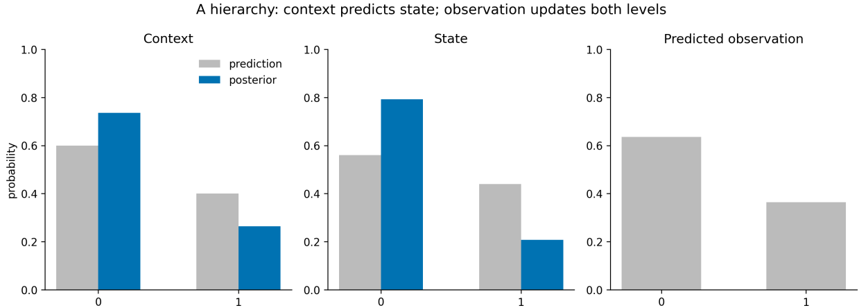
Figure 10: Prediction downward, inference upward. The context law induces a state prediction and an observation prediction. Conditioning on one observation updates both context and state using the same posterior joint, without discarding their dependence.
