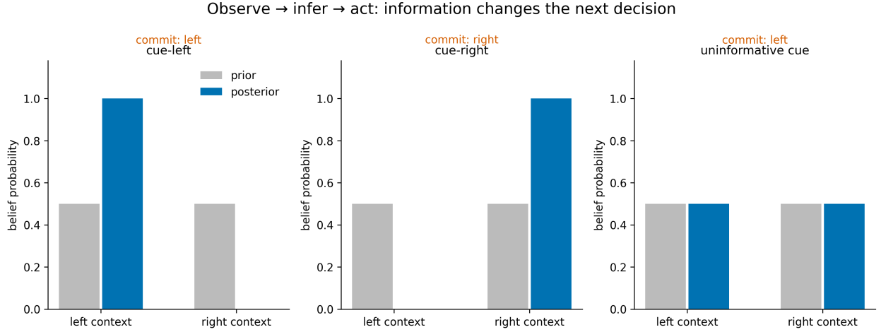
Figure 8: Observation changes the next decision. Informative cue-left and cue-right produce different posterior beliefs and opposite commitments. Replacing the cue with a state-independent coin leaves the prior unchanged and fails to produce an observation-sensitive commitment. Every panel comes from the same exact finite inference and action-selection core.
