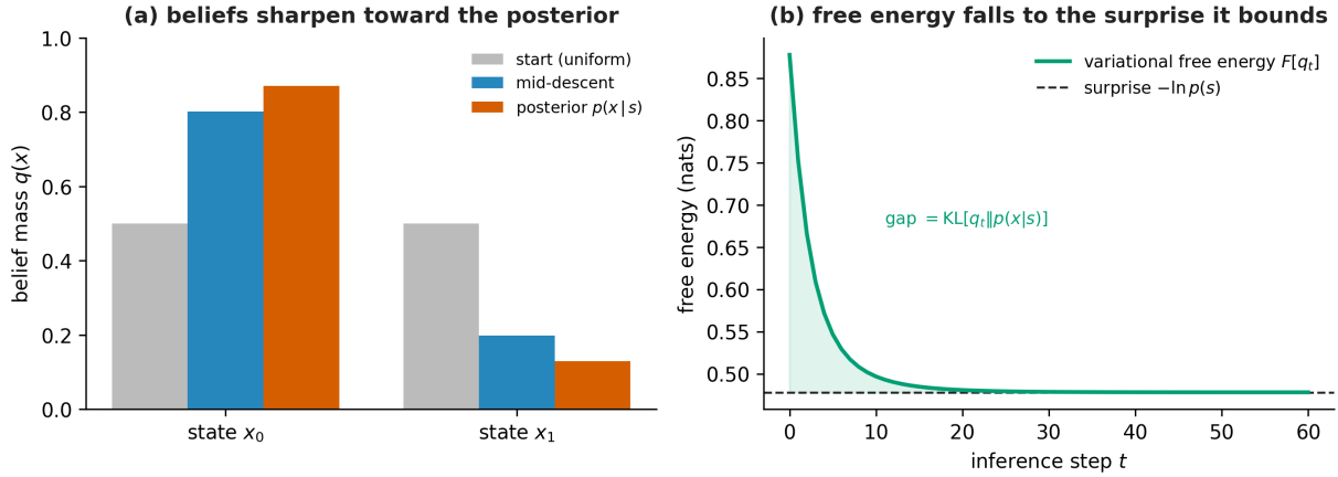
Figure 2: Perception as free-energy minimization. A two-state generative model (prior p(x) = (0.60, 0.40) ; likelihood favouring x_0 for the observed s ). (a) From a uniform starting belief, gradient descent on variational free energy drives the belief over hidden states to the exact Bayesian posterior p(x|s) (orange), passing through intermediate beliefs (blue) on the way. (b) Along the same descent the free energy F[q_t] falls monotonically to the surprise -\ln p(s) (dashed) that it bounds; the shaded gap is exactly KL[q_t || p(x|s)] , the belief’s error, which closes as inference completes. Minimizing free energy is Bayesian updating. Rendered deterministically by scripts/generate_belief_update_figure.py over the tested core in src/generative_model.py .
