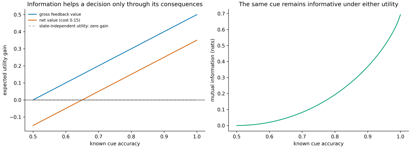
Figure 9: Decision value and information have distinct units. The left panel sweeps known cue accuracy for an observation-contingent commitment, its acquisition cost, and a state-independent utility counterexample. The right panel shows the same channel’s mutual information. Positive information does not imply positive instrumental value; a beneficial cue can also be too costly. Both panels use exact finite computation, not sampled performance estimates.
