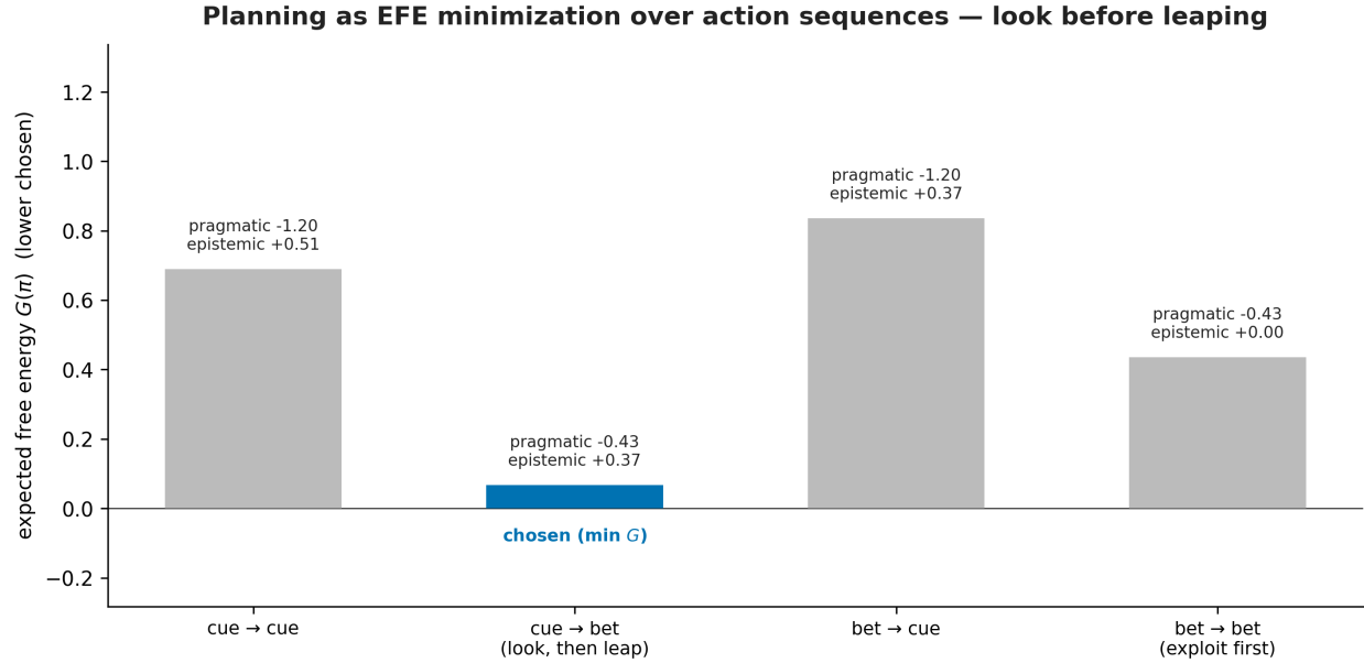
Figure 7: Finite sequence scoring. The four two-step sequences share a static hidden state. Cue-then-bet minimizes the declared terminal-preference minus history-information objective. The bet remains state-independent; the advantage is information scoring, not an observation-conditioned improvement in its payout.
