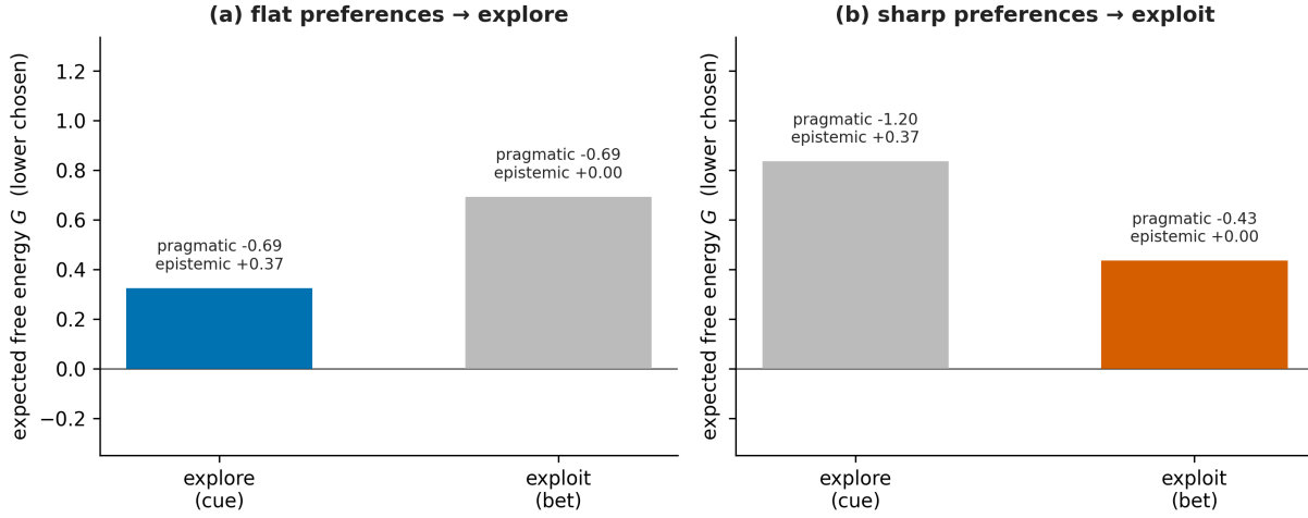
Figure 4: One rule yields explore and exploit. An agent uncertain between two contexts ( q(s) = (0.50, 0.50) ) chooses between an informative “cue” (epistemic value +0.37, preference-neutral) and a rewarding but uninformative “bet” (epistemic value 0). Bars are expected free energy G per action (lower is chosen); each is annotated with its pragmatic/epistemic split. (a) Flat preferences: the epistemic term dominates, so the agent explores (cue, G = 0.33 ). (b) Sharp preferences: the pragmatic term dominates, so the same \arg \min G rule exploits (bet, G = 0.43 ). A single rule; the balance of G ’s two terms — not a hand-coded switch — is what turns over between the panels. Rendered deterministically by scripts/generate_efe_figure.py over the tested core in src/expected_free_energy.py .
