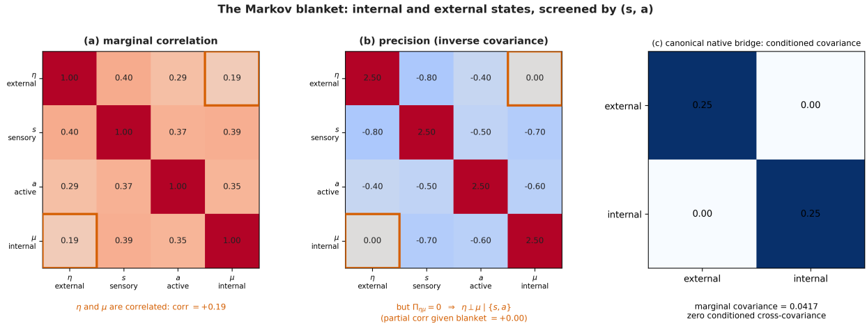
Figure 5: Marginal dependence, conditional independence. A jointly Gaussian world over external \eta , sensory s , active a , internal \mu , built with a zero \eta - \mu precision block. (a) Marginal correlation: \eta and \mu are correlated (0.19, highlighted) — they are statistically coupled through the blanket. (b) Precision (inverse covariance): the \eta - \mu entry is exactly 0, which in a Gaussian is conditional independence given the other variables — so \eta \perp \mu \mid \{s, a\} and the partial correlation given the blanket is 0. (c) The matched upstream canonical fixture has a diagonal conditioned endpoint covariance despite nonzero marginal coupling. The sensory and active states screen the internal states from the external world. Rendered deterministically by scripts/generate_markov_blanket_figure.py over the tested core in src/markov_blanket.py .
