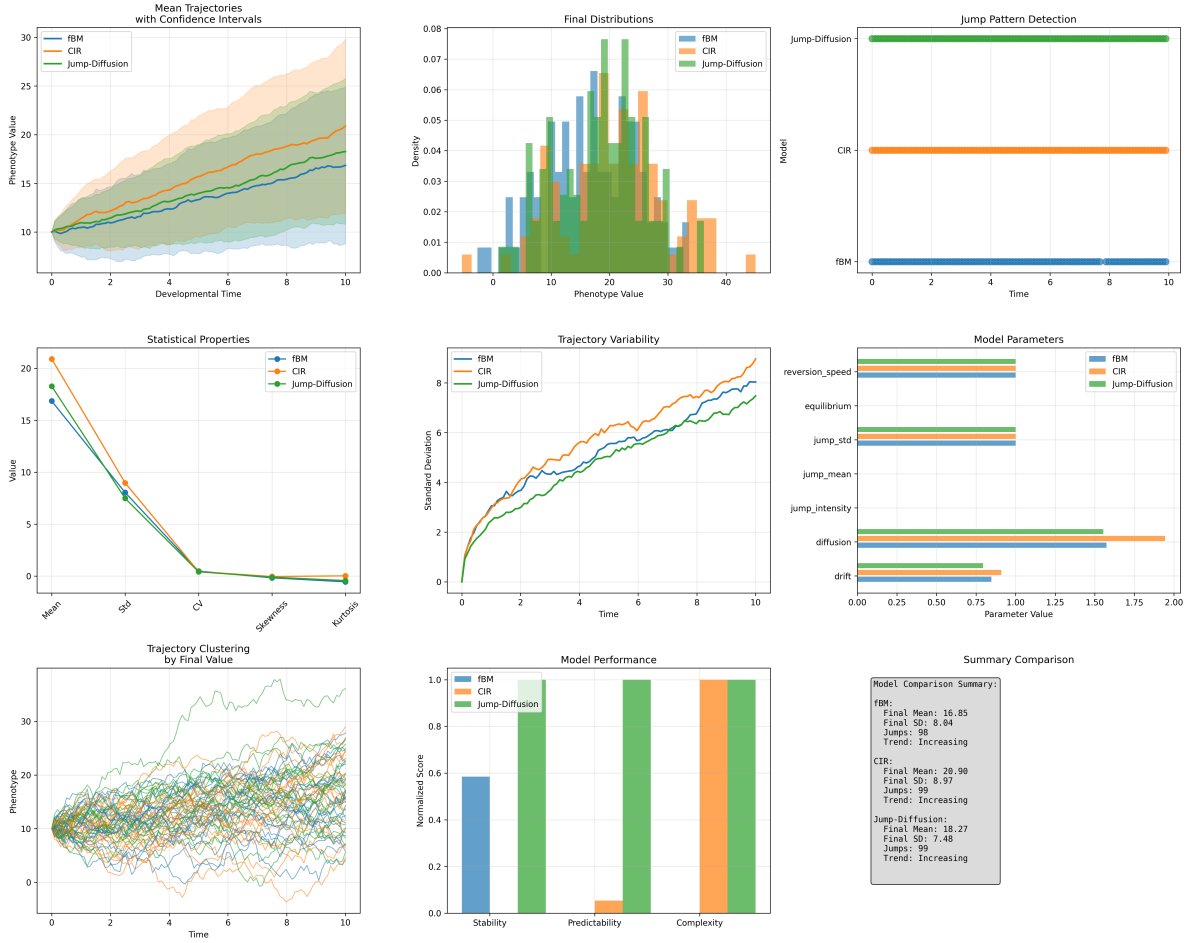
Figure 1: Comprehensive model comparison across stochastic processes showing trajectory patterns, statistical properties, parameter estimates, and performance metrics for fBM, CIR, and Jump-Diffusion models.
