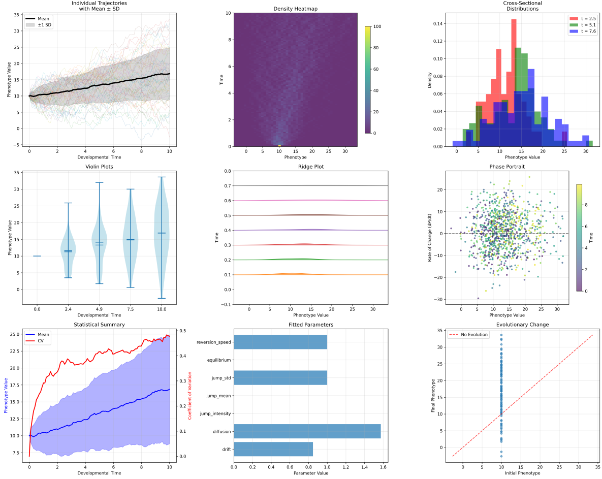
Figure 2: Comprehensive trajectory analysis of fBM model showing individual trajectories, density evolution, distribution comparisons, phase space dynamics, and statistical summaries across developmental time.
