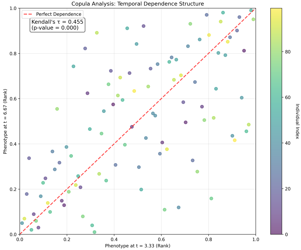
Figure 6: Copula analysis of synthetic developmental data showing rank-based scatter plot with Kendall's \tau = 0.45 ( p < 0.001 ) indicating significant positive trait dependence between early ( t=3.3 ) and late ( t=6.7 ) developmental phenotypes. The diagonal reference line represents perfect dependence, while points above/below indicate stronger/weaker coupling than expected under independence.
