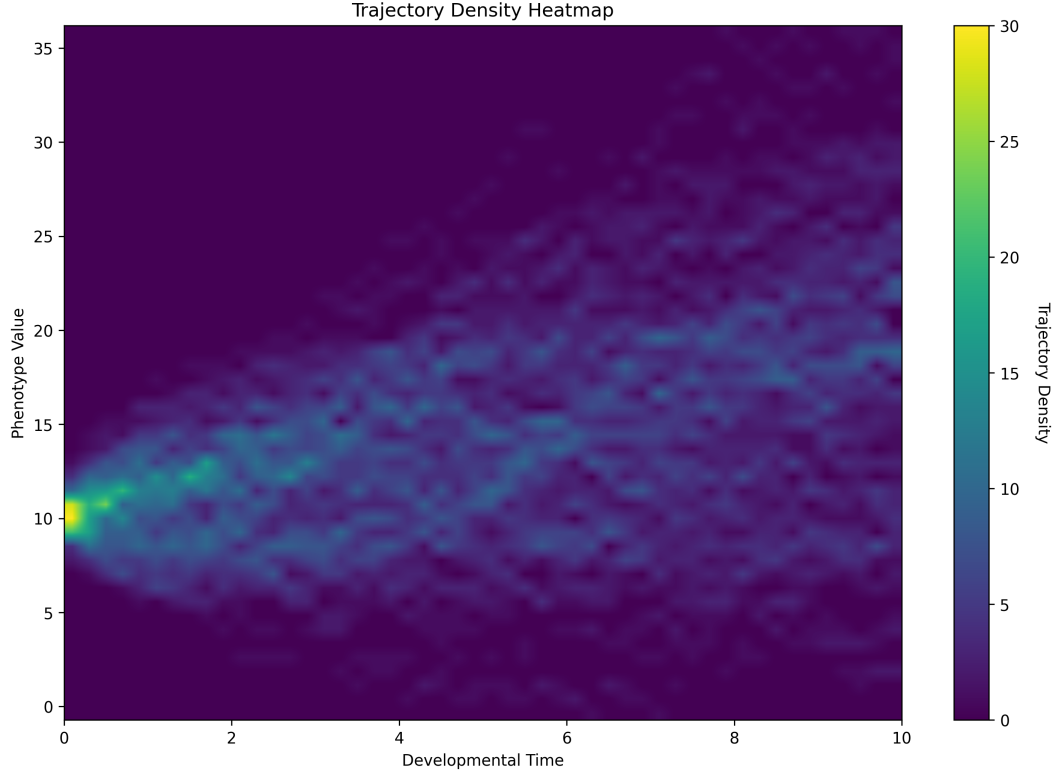
Figure 5: Individual model visualizations for Jump-Diffusion showing trajectory density heatmap.
