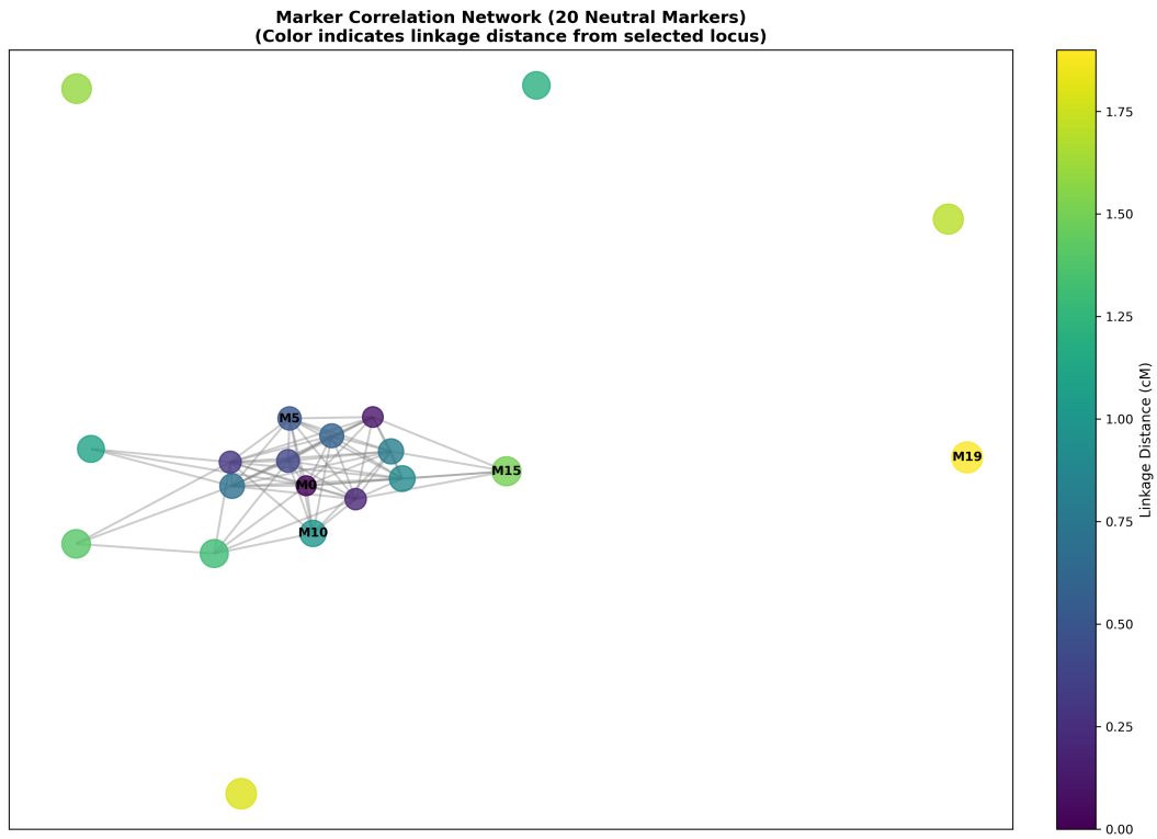
Figure 8: Network analysis of 20 neutral marker correlations during selective sweep, showing clusters of co-inherited variants. Markers are distributed from 0 to 2.0 cM from the selected locus, with color indicating linkage distance and network connections showing strong correlations ( >0.7 ).
