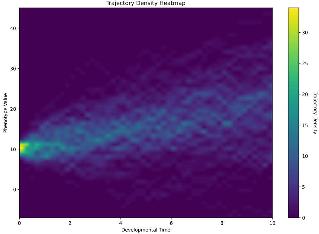
Figure 4: Individual model visualizations for CIR showing trajectory density heatmap.
