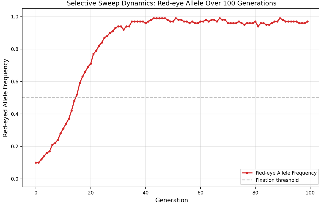
Figure 7: Selective sweep dynamics showing red-eye allele frequency evolution over 100 generations. The advantageous allele rises from 10% to near-fixation, following classic selective sweep dynamics under strong directional selection.
