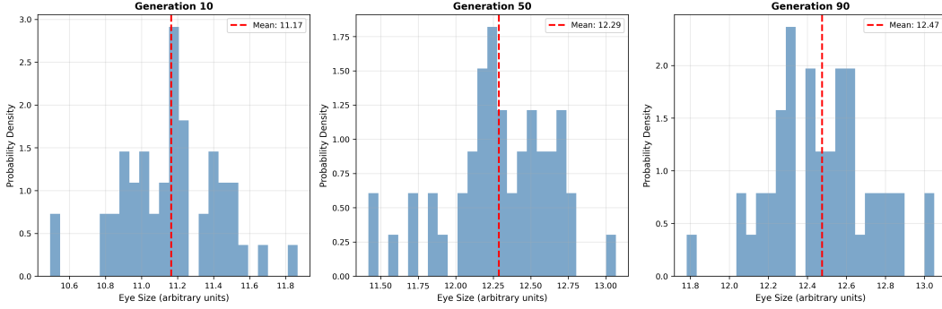
Figure 9: Cross-sectional distributions of eye size at different generations (10, 50, and 90) during the 100-generation selective sweep. As the advantageous red-eye allele increases in frequency, the mean eye size increases due to pleiotropy/linkage, demonstrating how selection on one trait (eye color) indirectly affects correlated traits (eye size).
