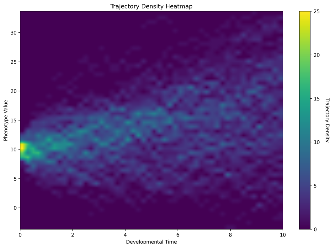
Figure 3: Individual model visualizations for fBM showing trajectory density heatmap.
