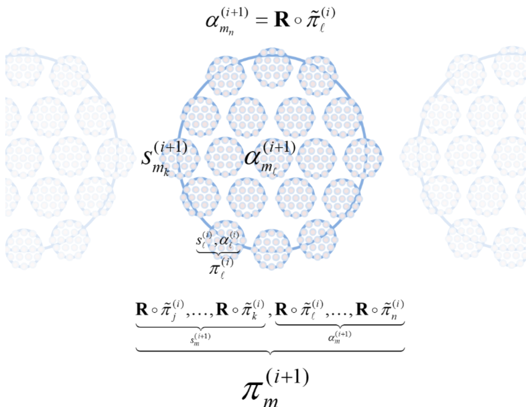
Figure 2. Schematic showing the hierarchical relationship between particles at scales i and i + 1 . For clarity, sensory and autonomous states are illustrated in blue and pink, respectively. Note that each variable is a (very large) vector state that itself is partitioned into multiple vector states. At scale i + 1 , each particle represents an ensemble (e.g., \pi_m^{(i+1)} is population m ), the elements of which are partitioned into autonomous and sensory subsets (e.g., \alpha_{m_n}^{(i+1)} is the n -th autonomous genotype from population m ). At scale i , each particle represents an element of an ensemble (e.g., \pi_\ell^{(i)} is the \ell -th
