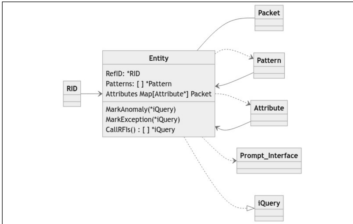
Figure 9. Entity component definition
