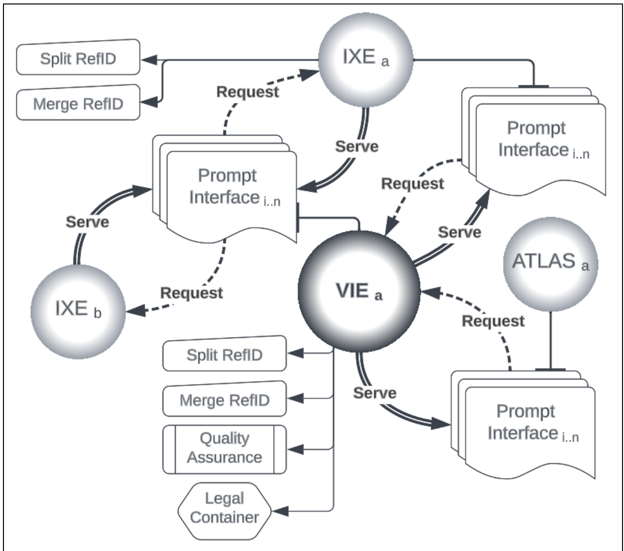
Figure 13. Schematic of interactions among Information Exchange Environments (IXE) and Verified Information Exchange Environments (VIE).
