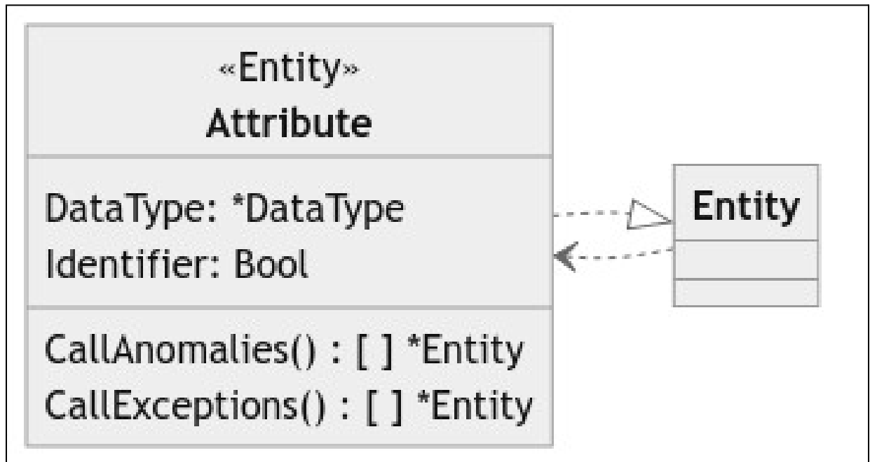
Figure 12. Attribute component definition.
