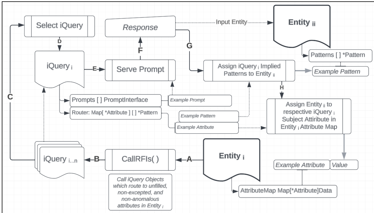
Figure 14. Representation of the role of iQuery objects in dynamic typing of Entity objects and routing of values resolving requests for information to Attributes.
