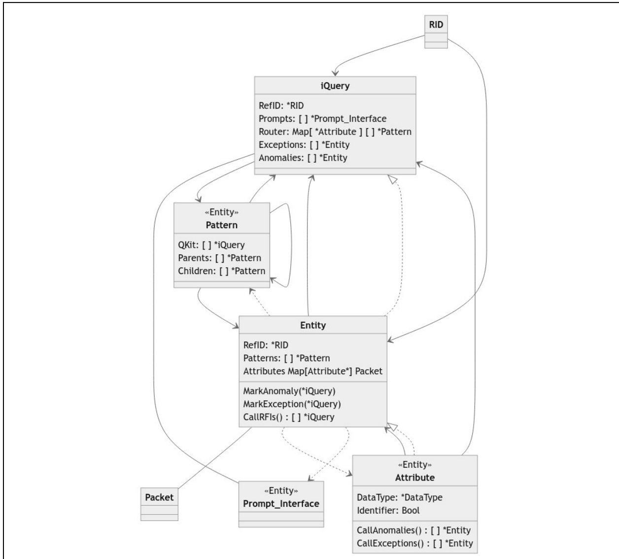
Figure 8. Representation of the full ATLAS system.
