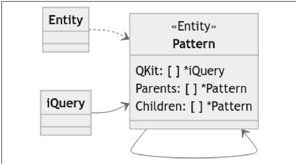
Figure 10. Pattern component definition.
