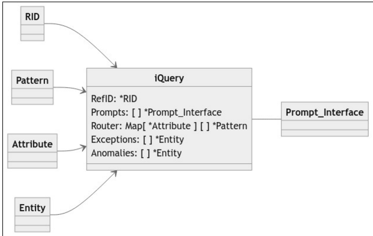
Figure 11. iQuery component definition.
