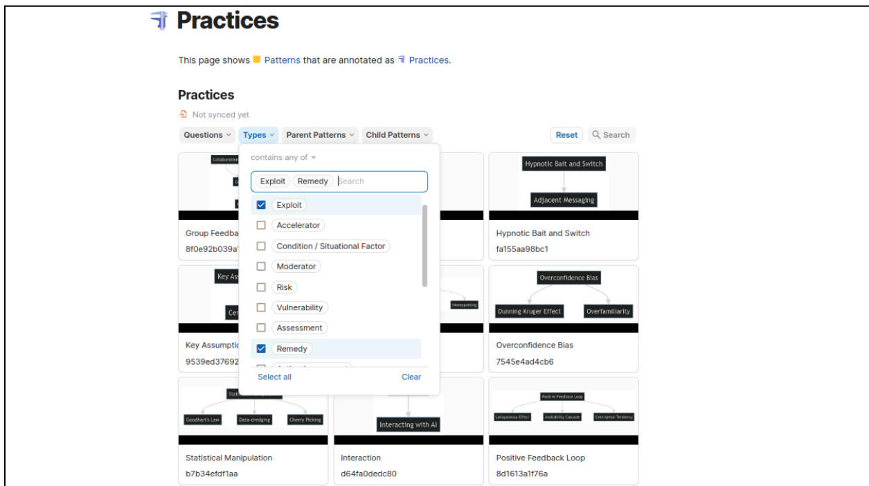
Figure 3. Snapshot of the ATLAS prototype page for patterns annotated as “Practices”. The patterns are further refined with the dropdown selection list, to patterns that have further been annotated as either Exploit or Remedy (these are practices that are either an exploit or remedy in a given setting).
