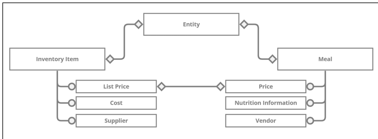
Figure 16. Representation of shared data despite varying schema and ontology.
